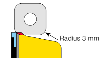
Spare Knives for Sidewall Planer 5549846 Radius 3 Blade (square) Pcs/Unit: 1
